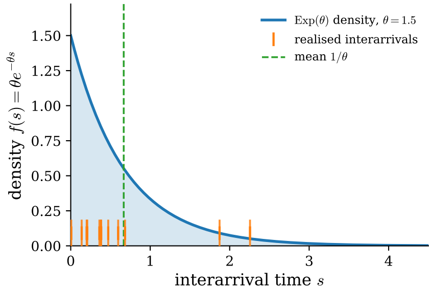
Interarrival law
